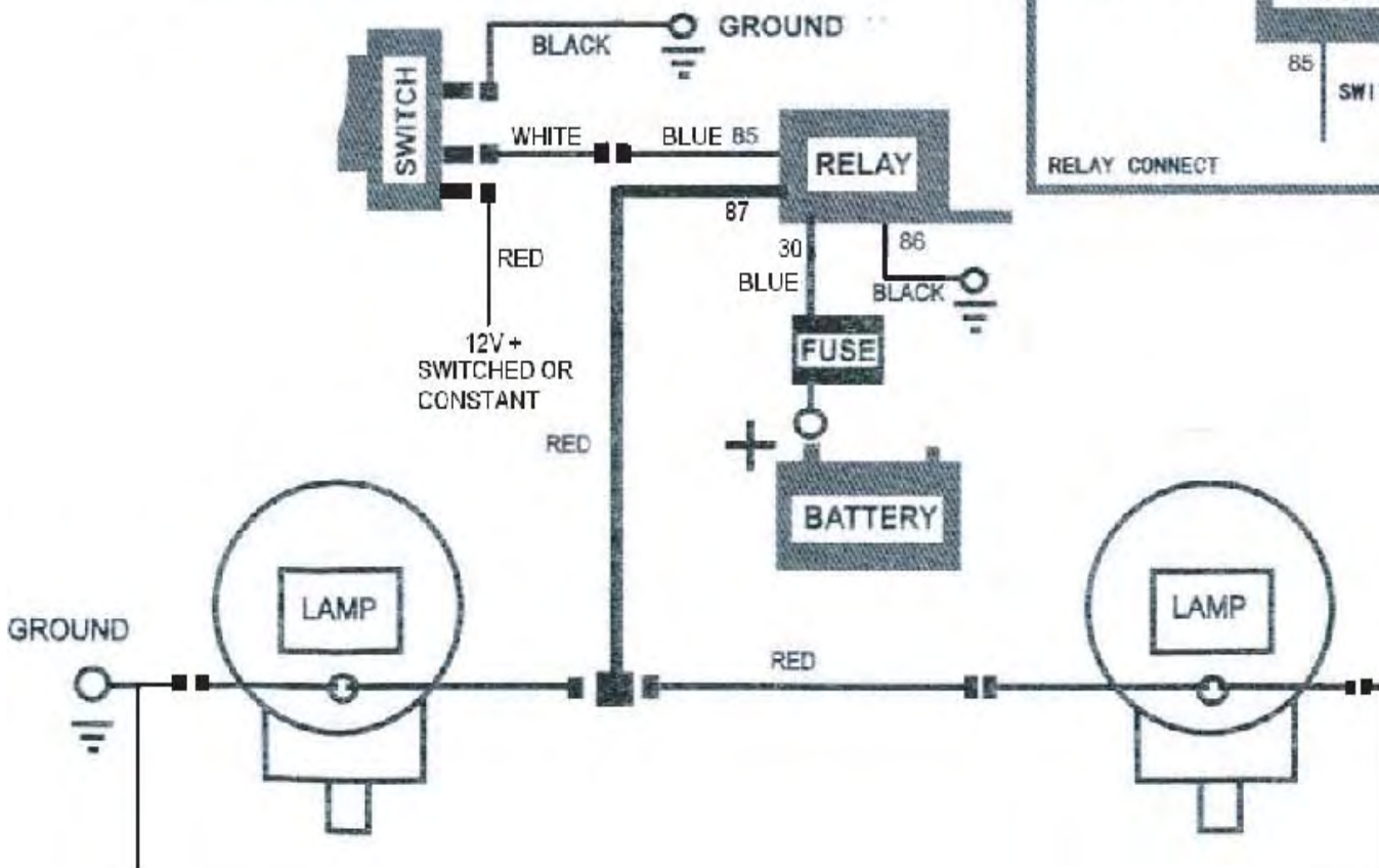
WIRE HARNESS DIAGRAM FOR 2 LIGHT
